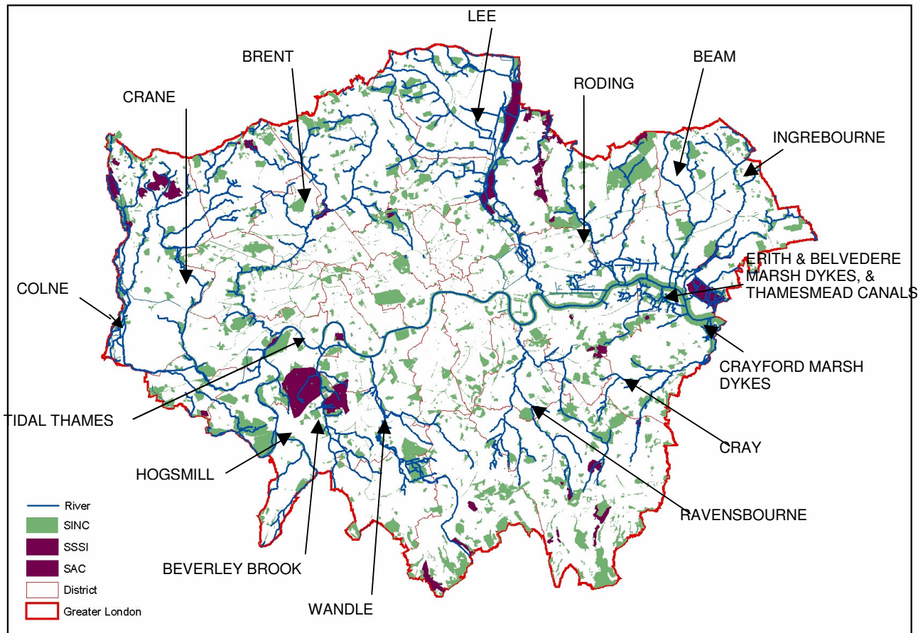
Figure 3: Map illustrating the location of river catchments along with the SSSIs, SACs and SINC within Greater London.
